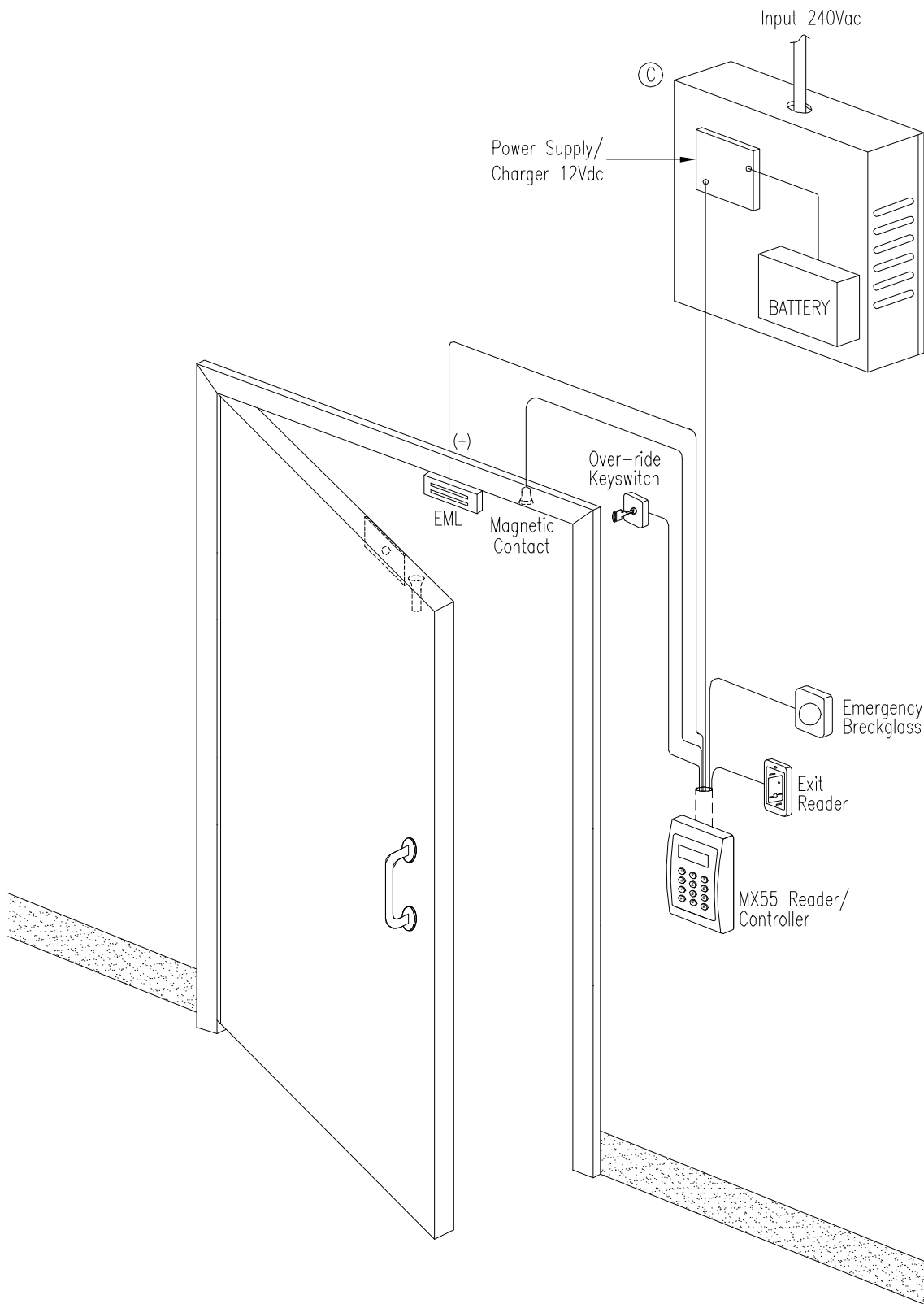
MX55 ACCESS CONTROL TYPICAL INSTALLATION LAYOUT WITH ELECTRO MAGNETIC LOCK
